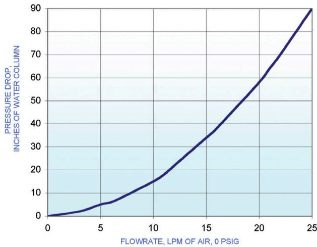
PRESSURE DROP vs. FLOW
